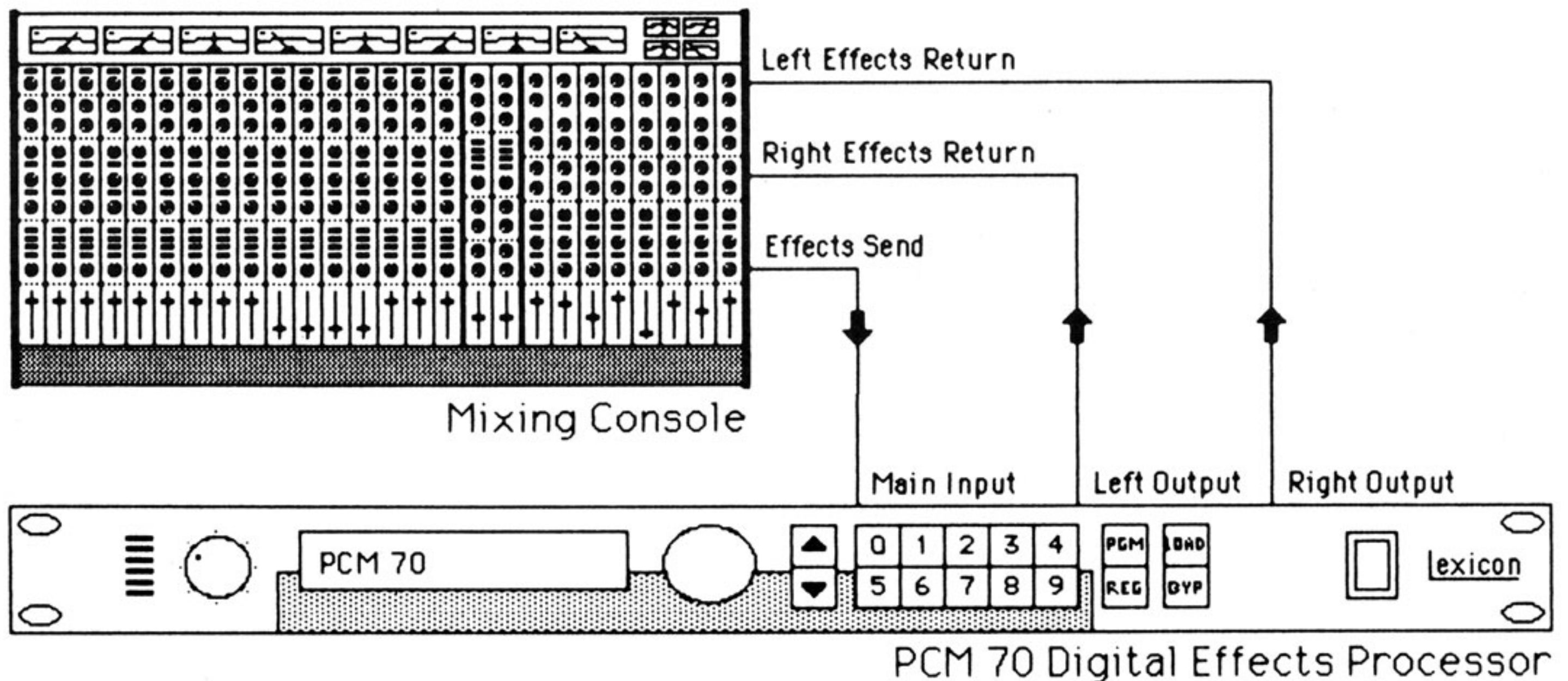
Figure 1.1. Connection to mixing console.
